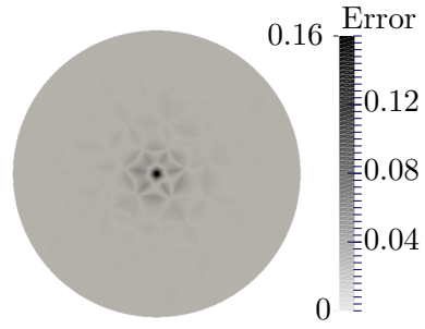
Figure 7: Error for 1/h \simeq 30 .
