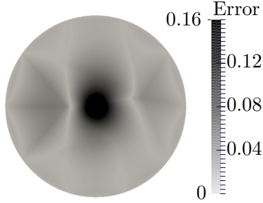
Figure 4: Error for 1/h \simeq 10 .
