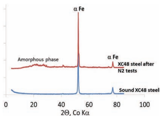
Fig. 4. X-ray traces of XC48 steel before (sound steel) and after series N2 (apparition of an amorphous phase).
