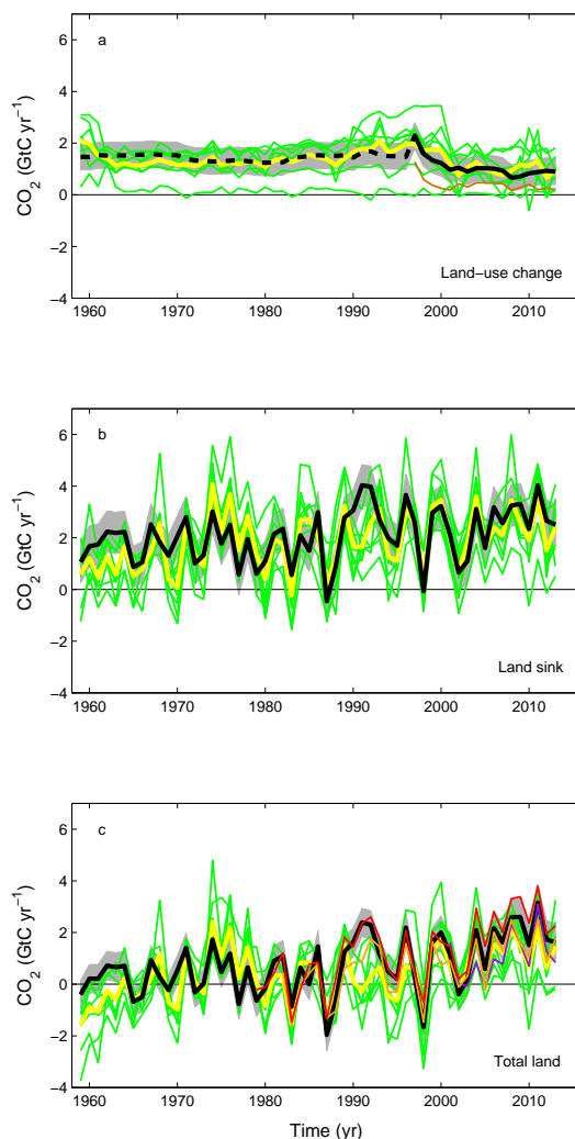
Figure 6. Comparison of the atmosphere–land CO 2 flux showing budget values of E_{LUC} (black line). (a) CO 2 emissions from land-use change showing individual DGVM model results (green) and the multi-model mean (yellow line), and fire-based results (brown); LUC data prior to 1997 (dashed black line) highlights the start of satellite data from that year. (b) Land CO 2 sink ( S_{LAND} ) showing individual DGVM model results (green) and multi-model mean (yellow line). (c) Total land CO 2 fluxes (sum of a + b) from DGVM model results (green) and the multi-model mean (yellow line), atmospheric inversions (MACC, v13.1 (Chevallier et al., 2005) in red; Rödenbeck et al. (2003) in orange; Peters et al. (2010) in purple; see Table 6), and the carbon balance from Eq. (1) (black). In (c) the inversions were corrected for the pre-industrial land sink of CO 2 from river input by adding a sink of 0.45 GtC yr -1 (Jacobson et al., 2007). This correction does not take into account the anthropogenic contribution to river fluxes (see Sect. 2.7.2).
