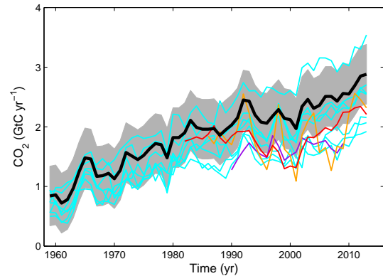
Figure 7. Comparison of the atmosphere–ocean \text{CO}_2 flux shows the budget values of S_{\text{OCEAN}} (black line), individual ocean models before normalisation (blue lines), and the three ocean data-based products (Rödenbeck et al. (2014) in orange, Landschützer et al. (2014) in red, and Park et al. (2010) in purple; see Table 6). All data-based products were corrected for the pre-industrial ocean source of \text{CO}_2 from river input to the ocean, which is not present in the models, by adding a sink of 0.45 \text{ GtC yr}^{-1} (Jacobson et al., 2007) in order to make them comparable to S_{\text{OCEAN}} . This correction does not take into account the anthropogenic contribution to river fluxes (see Sect. 2.7.2).
