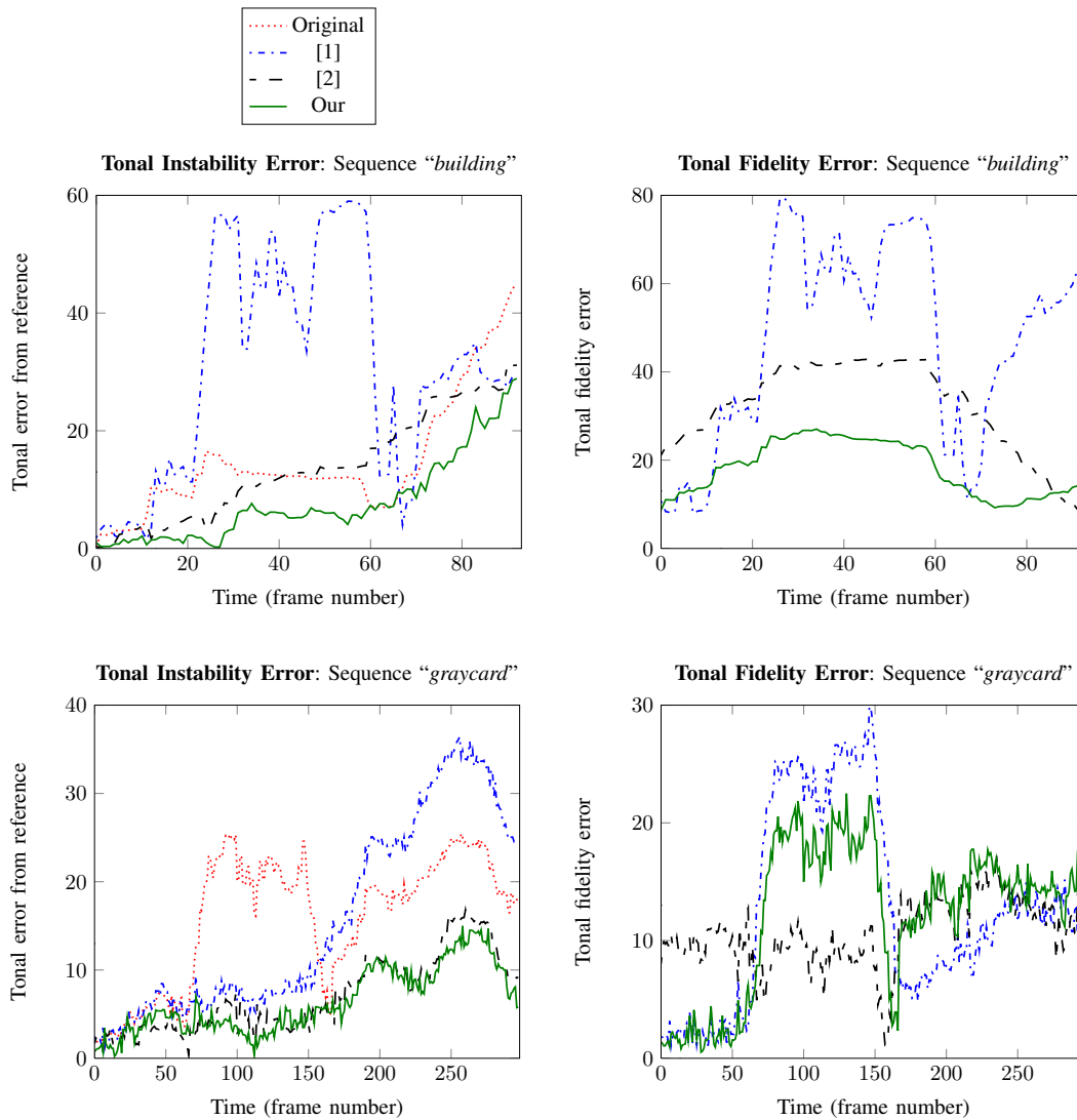
Fig. 7. Quantitative evaluation of the sequence "building" (top) and "graycard" (bottom). For each sequence, we show (i) the tonal instability error, computed as the color distance of a tracked patch to the reference (first) frame, and (ii) the tonal fidelity error, computed as the color distance at each instant, between the corrected frame and the original frame, which indicates the degree of fidelity between the original and the corrected sequence. The color distances are computed as the euclidian distance in perceptual color space CIELAB. Overall, our method compares favorably with the methods of [1] and [2], both in terms of reduction of tonal instability as in terms of fidelity to original colors.
