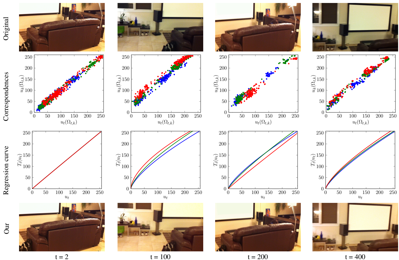
Fig. 3. Tonal stabilization of the sequence “sofa”. Top row: frames extracted from the original sequence, t = (2, 100, 200, 400) . Second row: plot of point correspondences between the original frame u_t and the keyframe u_k . Third row: estimated power law tonal transformation for each frame. Bottom row: same frames from top row, after tonal stabilization with our method. Note that objects appearing with different colors in the original sequence have the same color in our results. The color of the plotted points and curves correspond to the sRGB color channel (Red, Green, Blue) of the image.
