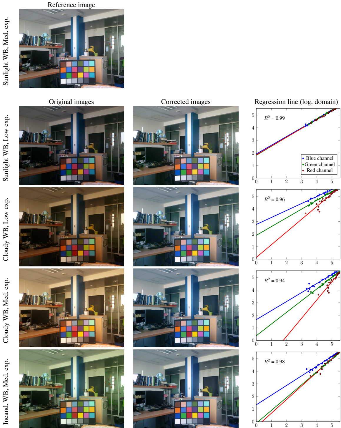
Fig. 2. Illustration of the goodness of fit of the proposed tonal transformation model. In this experience, a sequence of approximately registered images is taken from the same scene, and the color transformation is estimated from correspondent points extracted from the Macbeth color chart. On the first row, a reference image (keyframe u_k ) is shown. For the following second to fifth rows, on the left column, tonally unstable images ( u_t ) taken with different exposures and white balance are shown. On the middle column, the color corrected images are shown, where it can be noted that tonal instability is largely reduced. Finally, on the right column, the extracted points from the color chart and the estimated regression lines are plotted in the logarithmic domain. The x -axis corresponds to \log u_t^c(\Omega_p) , while the y -axis corresponds to \log u_k^c(\Omega_p) for the plotted points and T_t^c(\log u_t^c(\Omega_p)) for the plotted lines, where \Omega_p is the set of color chart coordinates. The regression line has a close fit to the color points, reminding that R^2 values which are close to 1 are an indication of a good fit.
