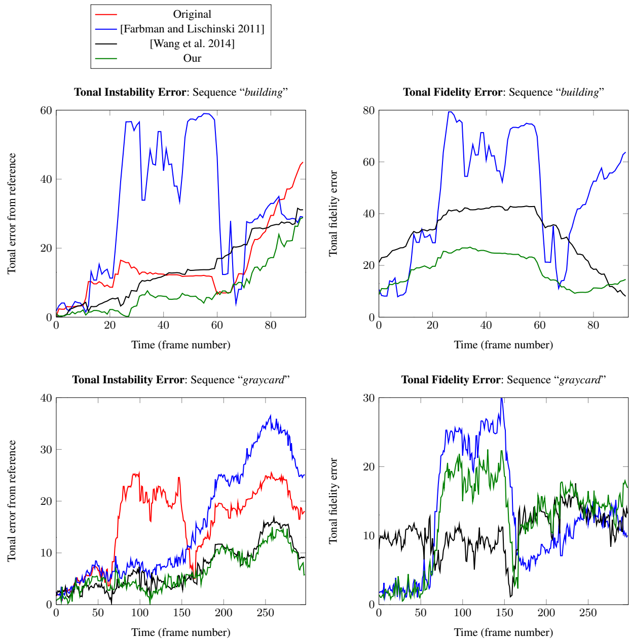
Fig. 7. Quantitative evaluation of the sequence “building” (top) and “graycard” (bottom). For each sequence, we show (i) the tonal instability error, computed as the color distance of a tracked patch to the reference (first) frame, and (ii) the tonal fidelity error, computed as the color distance at each instant, between the corrected frame and the original frame, which indicates the degree of fidelity between the original and the corrected sequence. The color distances are computed as the euclidian distance in perceptual color space CIELAB. Overall, our method compares favorably with the methods of [Farbman and Lischinski 2011] and [Wang et al. 2014], both in terms of reduction of tonal instability as in terms of fidelity to original colors .
