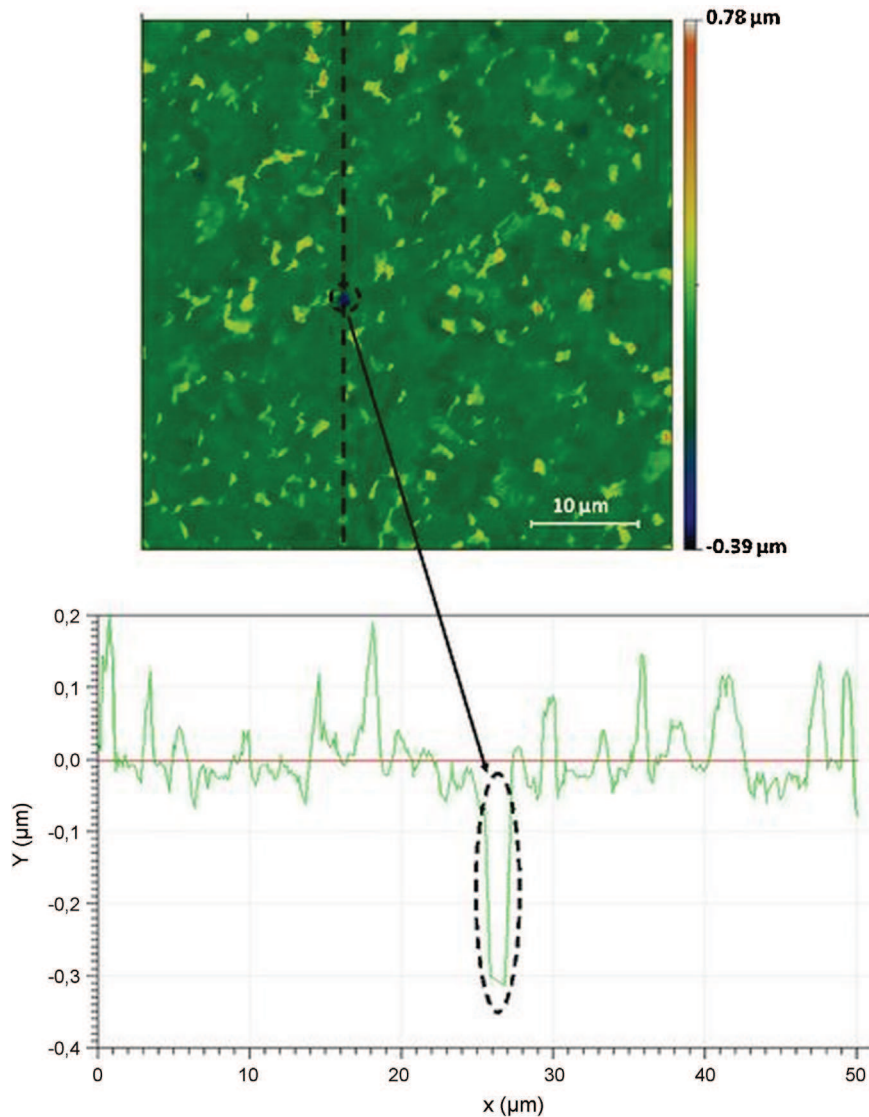
Fig. 6. SPM surface mapping and profile of polished then pickled sample ( \text{HNO}_3 -HF (20–2 w%) solution, 20 °C, 200 s) showing a pit.
