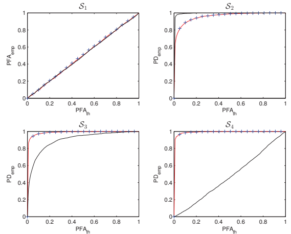
Fig. 3. Empirical ROCs of the tests (13) (red lines), (17) (blue crosses) and the test studied in [8] (black lines) for \mathcal{S}_1 to \mathcal{S}_4 .
