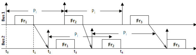
Fig. 6. The immediate forwarding strategy
