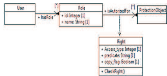
Fig. 4. RBAC pattern (adopted from [1])
