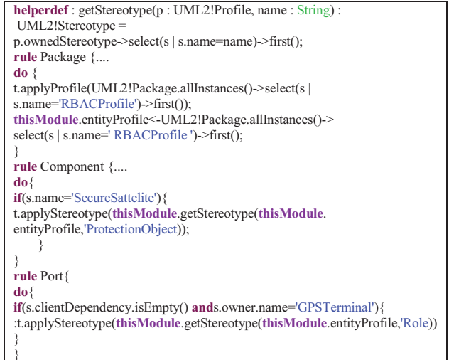
Fig 7. Part of RBAC pattern application rules
