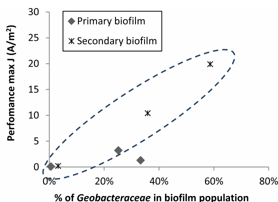
Fig. 5. Correlation between the maximal current densities and the percentage of Geobacteraceae in bioanode microbial communities.
