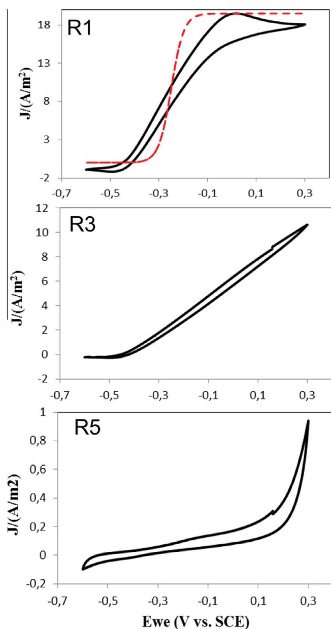
Fig. 2. Catalytic voltammetries recorded on day 37. (R1): biofilm formed in synthetic medium with activated sludge inoculum; (R3): biofilm formed in wastewater with activated sludge inoculum; (R5): biofilm formed in wastewater without the activated sludge inoculum. The dotted sigmoid curve in the R1 CV represents the Nernst-Michaelis equation.
