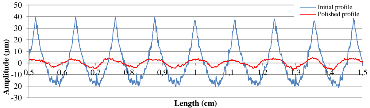
Fig. 2: Optimal topography profile of the experimental design (85 % of surface roughness reduction)
