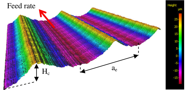
Fig. 2. Characteristics parameters of milled surface, measured by focal variation microscopy.
