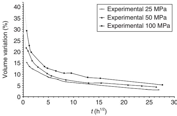
Figure 3 Experimental curves of volume variations during CO 2 desorption in PVF 2 for high-pressure tests. (Reprinted from [35], Fig. 1).
