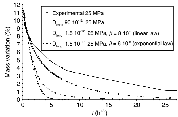
Figure 10 Desorption kinetics for a high-pressure test (25 MPa): comparison between Fick's law ( D_{\text{short}} of 90 \times 10^{-12} \text{ m}^2 \cdot \text{s}^{-1} ), linear and exponential laws ( D_{\text{long}} of 1.5 \times 10^{-12} \text{ m}^2 \cdot \text{s}^{-1} ).
