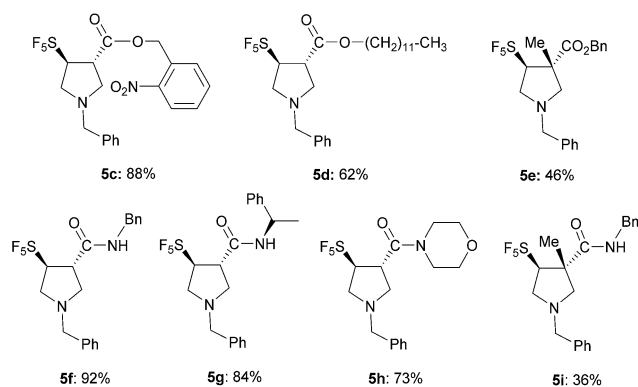
Fig. 1 Scope of the 1,3-dipolar cycloaddition using precursor 4 of azomethine ylide. 11
