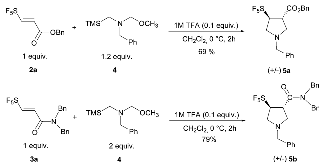
Scheme 2 Synthesis of pentafluorosulfonyl pyrrolidines 5a and 5b .
