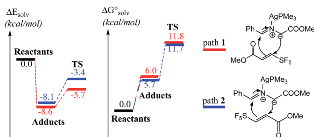
Fig. 2 Regiochemistry according to \Delta E_{\text{Solv}} and \Delta G^\circ_{\text{Solv}} viewpoints for the SF 5 -ester compound 12.
