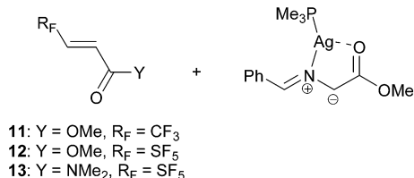
Scheme 3 Model systems 11–13 for the theoretical study.
