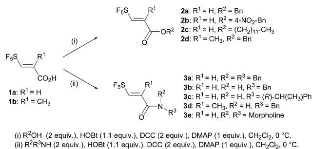
Scheme 1 Synthesis of pentafluorosulfanyl-substituted esters 2 and amides 3 .
