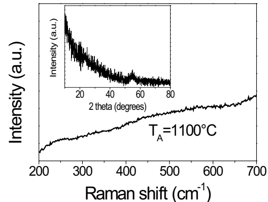
Figure 2 Raman spectrum on fused silica sample annealed at 1100 ^\circ\text{C} . The inset showed XRD pattern of Tb-doped film annealed at 1100 ^\circ\text{C} .
