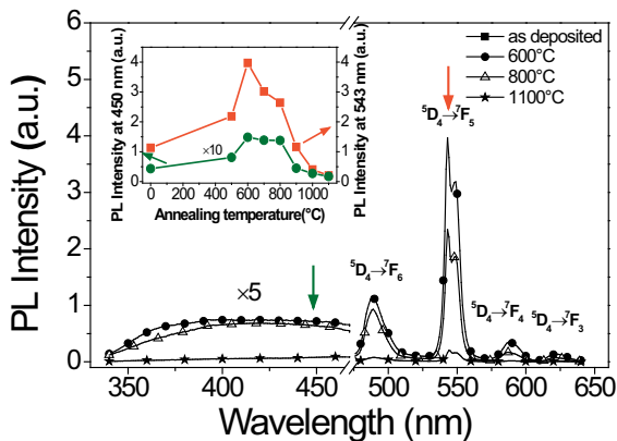
Figure 3 PL spectra excited at 325 nm for different annealing temperature. Inset is PL intensities at 543 nm ( Tb^{3+} ) and 450 nm (band tail states) as a function of the annealing temperature.
