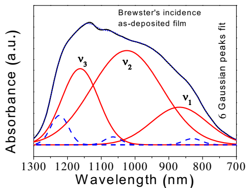
Figure 1 FTIR spectrum of as-deposited film recorded at Brewster angle ( 65^\circ ).
