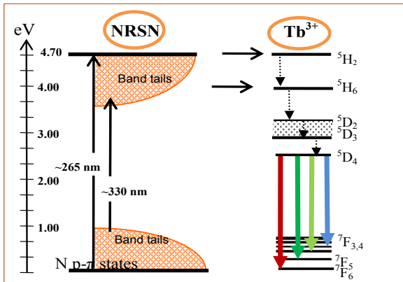
Figure 5 Schematic band diagram of the Tb-NRSN film with a mechanism proposed to explain the PL in the NRSN film.
