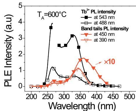
Figure 4 PLE spectra of 600 °C-annealing sample monitored at 543 nm, 488 nm ( Tb^{3+} related) and 450 nm and 390 nm (band tails).
