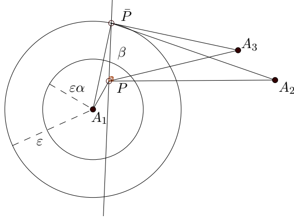
Figure 6: Construction of the modified deformation.
