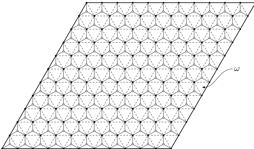
Figure 3: Alternate Delaunay triangulation.
