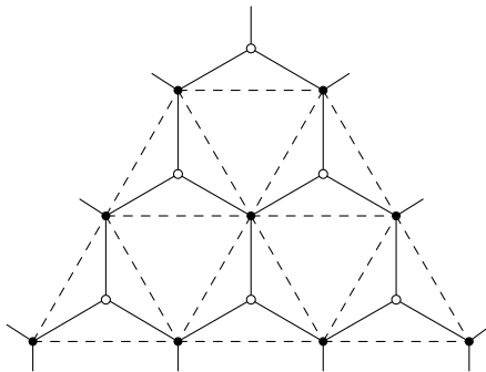
Figure 1: \bullet : type 1 nodes, \circ : type 2 nodes
