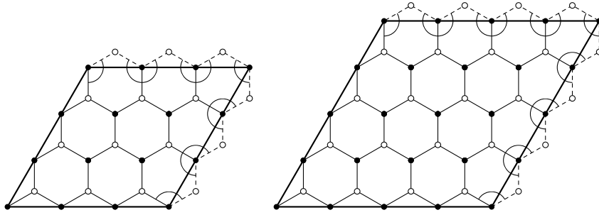
Figure 7: The cells 3Y and 4Y with added phantom nodes and angles.
