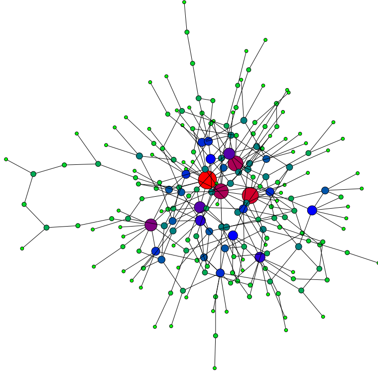
FIGURE 1: The largest connected component of a RPLG(n, t) for n = 300 and t = 2.9 . The component has 210 nodes (whose size is depicted proportional to their degree) and 268 edges. The maximum degree is 23.
