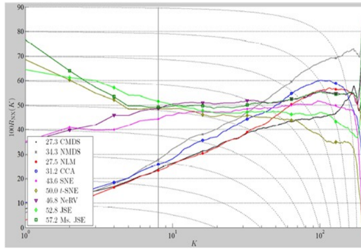
Figure 1: Quality curves of R_{NX} function on the square root of the data
