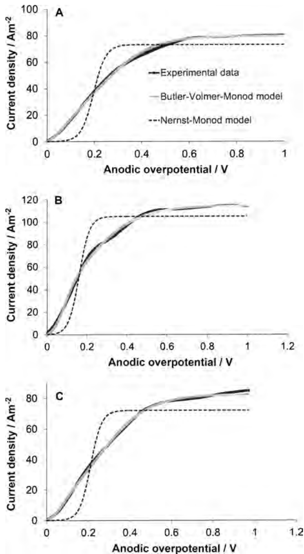
Figure 2. Forward scan (1 mV s -1 ) voltammetry for three bioanodes formed in parallel by 25 days of polarisation at 0.1 V/SCE at a NaCl concentration of 45 g L -1 (triplicates). The experimental curves were plotted by taking the OCP as the origin of potentials and then fitted with the Nernst-Monod and the Butler-Volmer-Monod equations.
