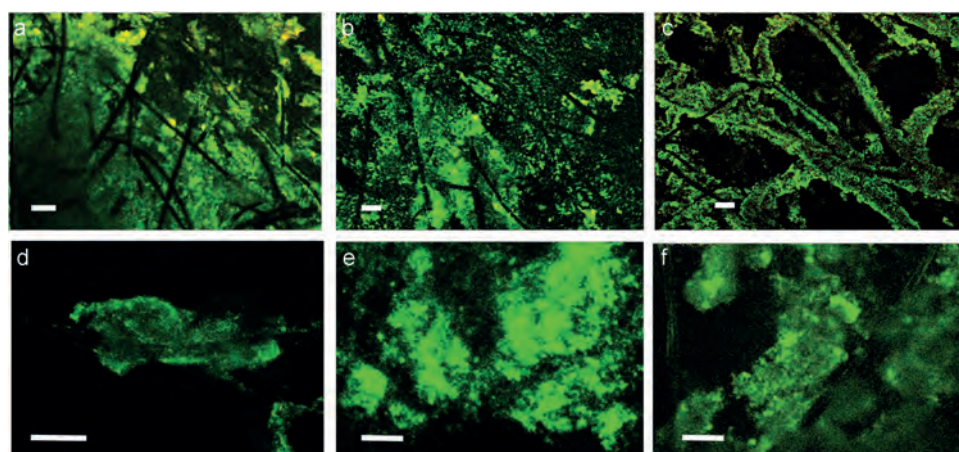
Figure 4. Confocal laser scanning microscope images of bioanodes stained with Bacterial Gram staining (a–c) and NanoOrange (d–f). Bioanodes were formed at NaCl concentrations of 30 g L -1 (a, d), 45 g L -1 (b, e) and 60 g L -1 (c, f). Scale bars: 20 μm. Projection of Z sections (1 μm step) through a) 25 μm, b) 46 μm, c) 1 μm, d) 21 μm, e) 22 μm and f) 17 μm. Sheathing of fibres increased with increasing NaCl concentration and the biofilm became more rarefied in the interstitial spaces between adjacent graphite fibres.
