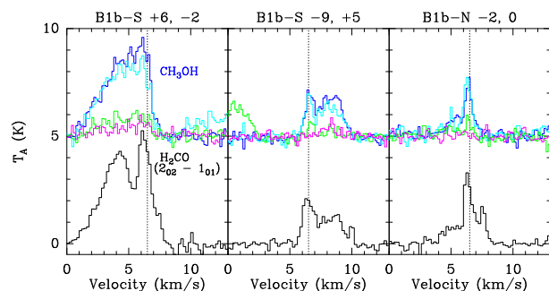
Fig. 2. Examples of CH 3 OH and H 2 CO spectra towards the B1b-S and B1b-N outflows. The H 2 CO(2 02 - 1 01 ) line is shown in black. The four detected CH 3 OH lines are shown in color: blue 3 0 -2 0 E, cyan 3 -1 -2 -1 E, green 3 0 -2 0 E, and purple 3 2 -2 2 E. They have been vertically shifted by 5 K for clarity.
