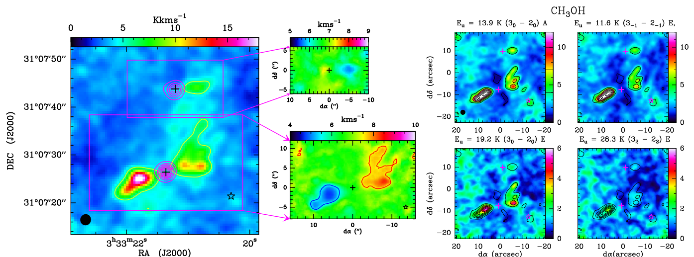
Fig. 1. Left: Integrated intensity (from 0 to 14 \text{km s}^{-1} ) and velocity field of the \text{H}_2\text{CO}(2_{0,2} - 1_{0,1}) line. Purple contours show the continuum emission at 145 GHz. The plus signs indicate the positions of B1b-N and B1b-S. The star shows the position of B1b-W. The black ellipse shows the beam size. The small panels show the centroid velocity towards B1b-N (top) and B1b-S (bottom) in \text{km s}^{-1} . Right: Integrated intensity images (from 1.5 to 12.5 \text{km s}^{-1} ) of the four \text{CH}_3\text{OH} lines detected towards B1b: from left to right and top to bottom: 3_0 - 2_0 A, 3_{-1} - 2_{-1} E, 3_0 - 2_0 E and 3_2 - 2_2 E. The intensity scale in \text{K km s}^{-1} is given by the color bar on the right. Contours of the 3_0 - 2_0 A line are superimposed in all plots, ranging from 1 to 20 \text{K km s}^{-1} with a step of 3 \text{K km s}^{-1} . Offsets are given relative to the pointing center given in Table 1.
