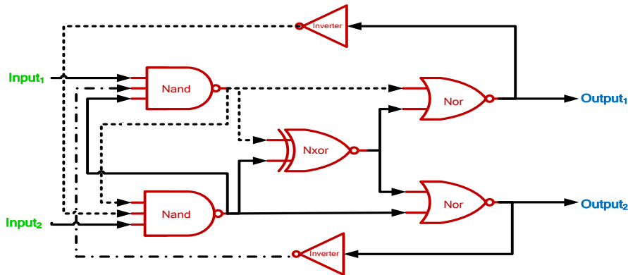
Arbiter Concurrency Primitive 49
