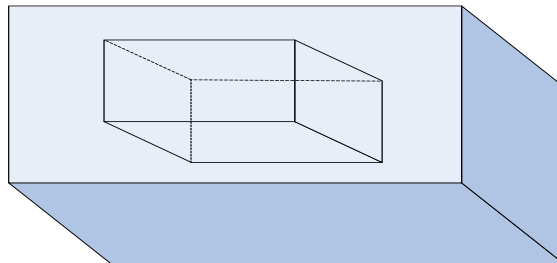
Counterexample to Euler's Formula
