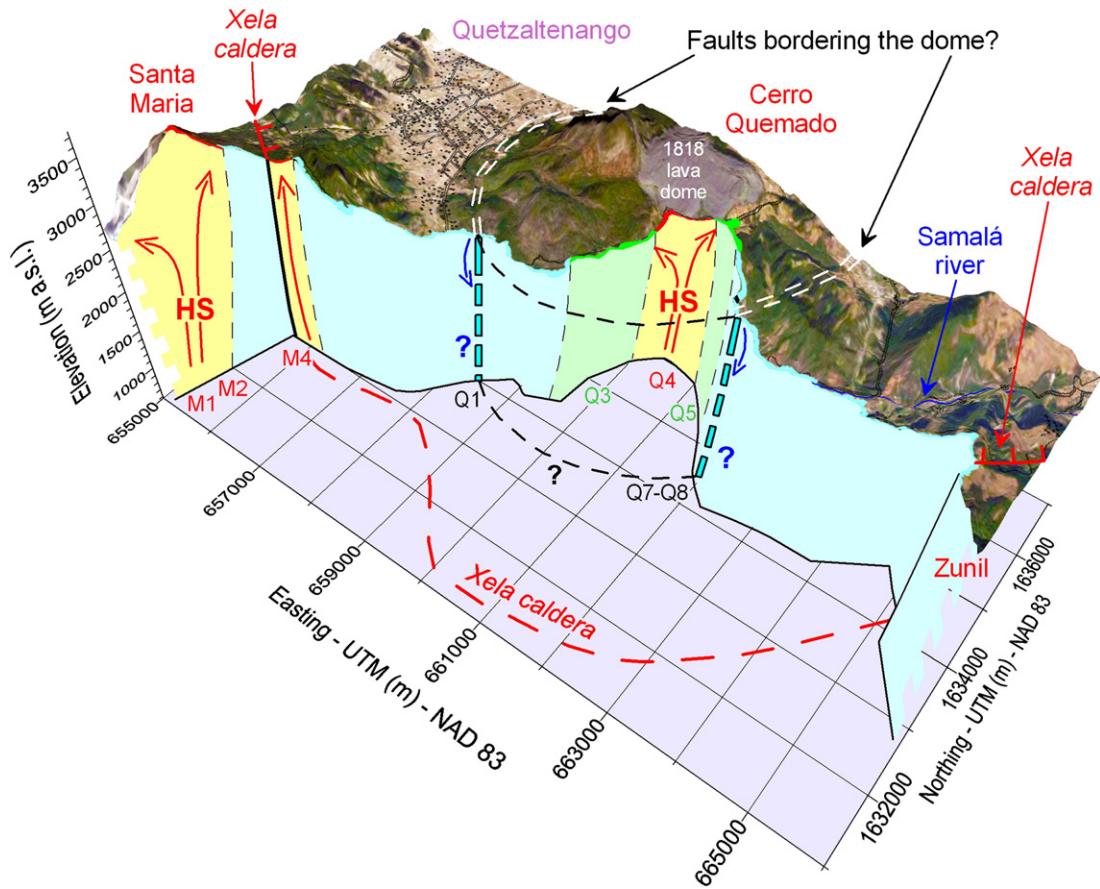
Fig. 6. Landsat image overlapped on a 3D (10 × 10 m grid) digital elevation model of the Santa María–Cerro Quemado–Zunil area. Interpretation of fluid flows has been reported with different colors and arrows along the 16.880 km-long profile, highlighting the main structural discontinuities constraining fluid flows. Symbols are the same as in Fig. 5. (For interpretation of the references to colour in this figure legend, the reader is referred to the web version of this article.)
