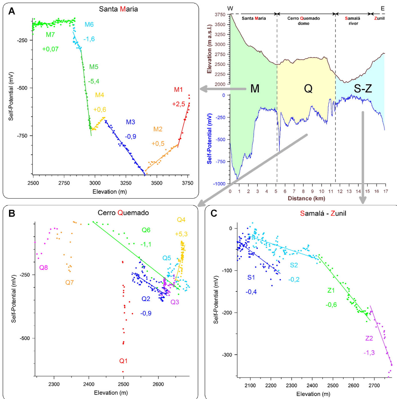
Fig. 4. Self-potential signal versus elevation for: Santa María volcano area (A), Cerro Quemado dome complex (B), and Samalá River and Zunil volcano area (C). Letters represent subdivisions as defined in Fig. 3. Color-coded numbers represent values of self-potential/elevation gradients for select subdivisions (unit: mV/m). Four positive self-potential/elevation gradients (M1, M2, M4, and Q4) and three short wavelength minima (Q1, Q7, and Q8) have been highlighted. Their significance is discussed in the text. (For interpretation of the references to colour in this figure legend, the reader is referred to the web version of this article.)
