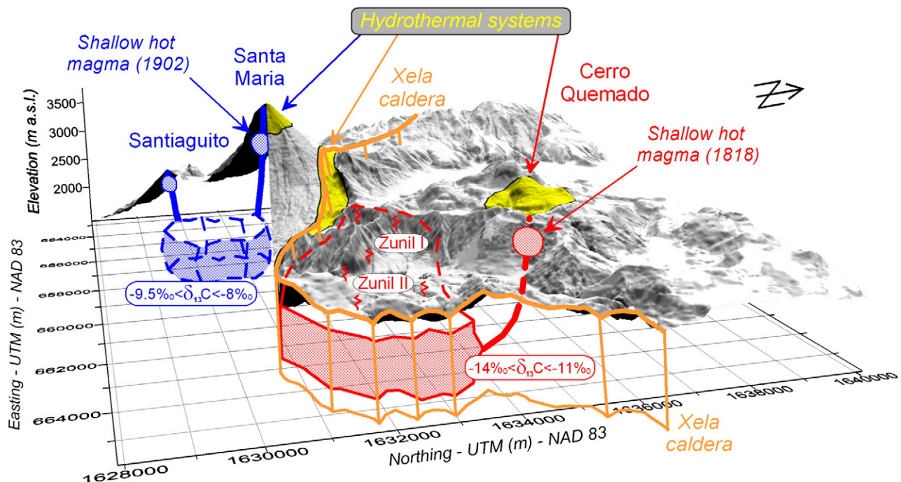
Fig. 7. Large-scale 3D interpretation of hydrothermal fluid flows with potential heat sources distribution to explain the self-potential data obtained during the field campaign, and the water carbon isotopic values from Walker et al. (2006). Important: depth and size of heat sources not at scale.
