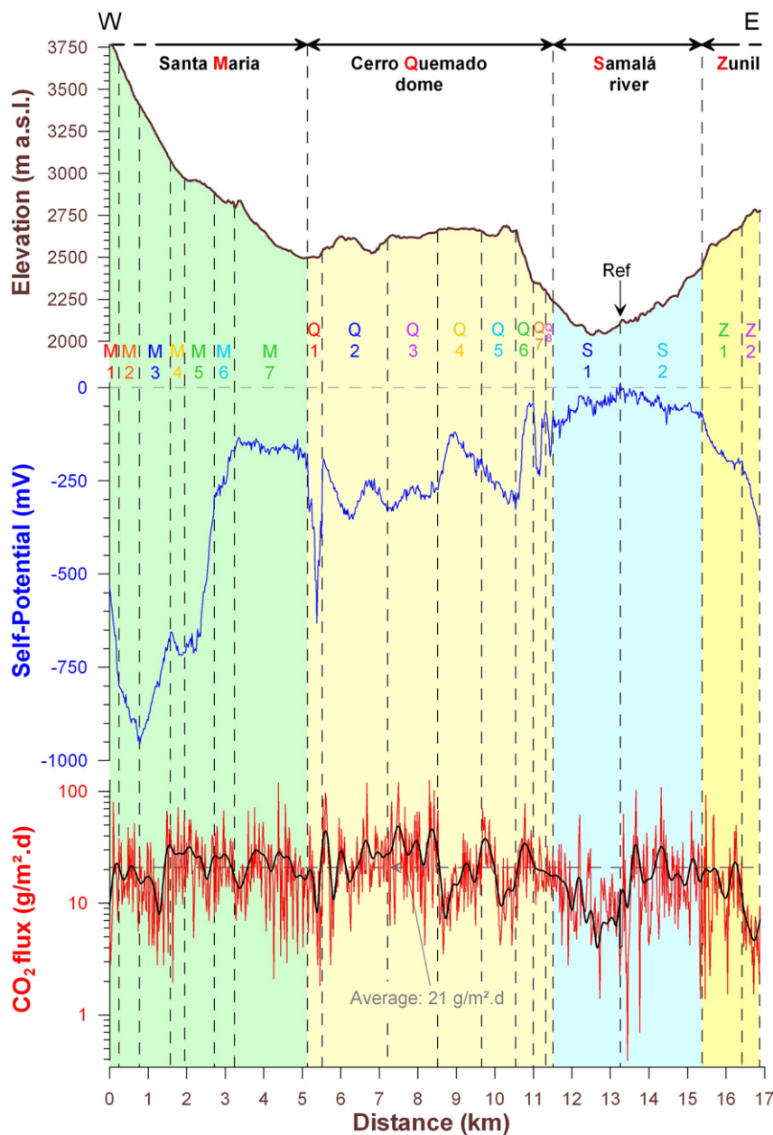
Fig. 3. Elevation (brown), self-potential (blue), and soil CO 2 flux (red) versus distance along the studied profile. The black curve represents soil CO 2 flux data smoothed by a FFT-low pass filter. The CO 2 signal does not show any significant anomaly, while four distinct subdivisions can be distinguished via self-potential: M1–7, Q1–8, S1–2, and Z1–2, termed Santa María, Cerro Quemado, Samalá River, and Zunil, respectively. See details in the text. “Ref” refers to the self-potential reference measured on the border of Samalá River. (For interpretation of the references to colour in this figure legend, the reader is referred to the web version of this article.)
