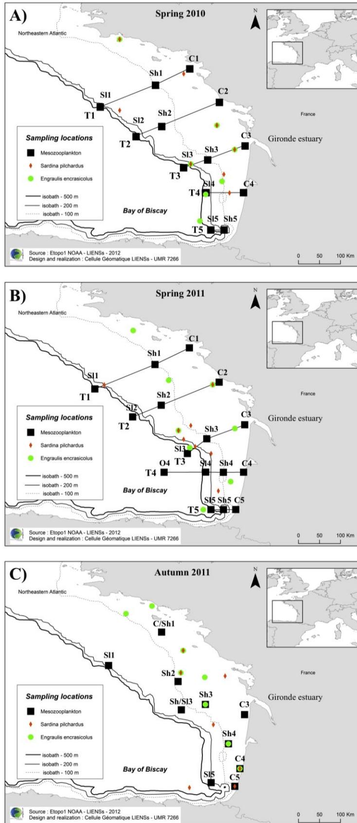
Figure 1. Maps of the study area (Bay of Biscay), with transects realised from the coastline to the slope and stations selected for plankton sampling for each of the 3 periods considered in this study: A) Spring 2010, B) Spring 2011 and C) Autumn 2011. Trawls of fish sampling are also indicated. T = Transect; C = Coast; Sh = Shelf; SI = Slope; O = Oceanic.
