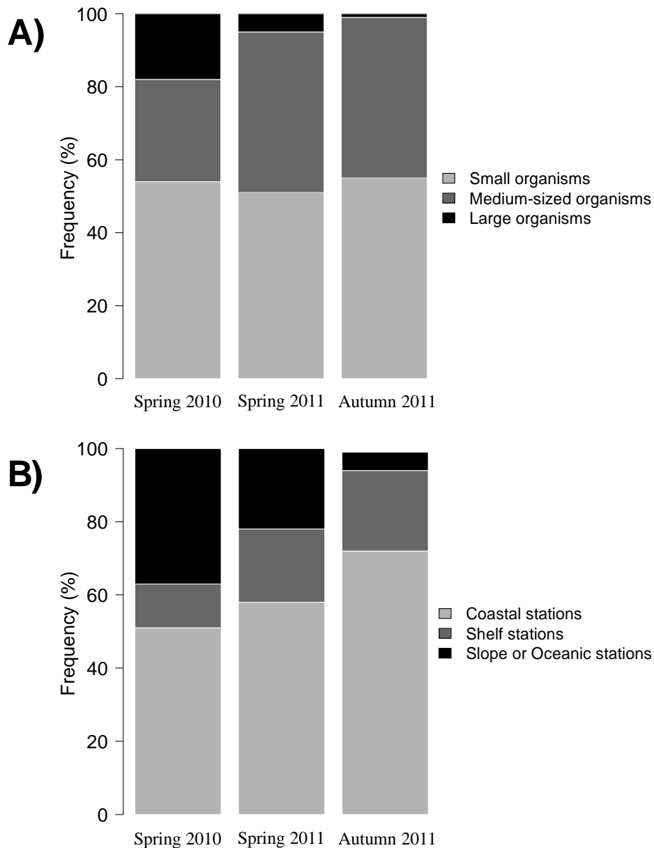
Figure 4. Stacked bar charts presenting a the frequency of identified organisms belonging to small, medium-sized or large organisms within each of the three periods considered in this study, all stations considered together over the Bay of Biscay; b the frequency of organisms identified in coastal stations, stations from the shelf or stations from the slope and oceanic stations within each of the three periods considered in this study, all sizes considered together. Only organisms belonging to ‘dominant taxa’ were taken into account for both histograms (see text).
