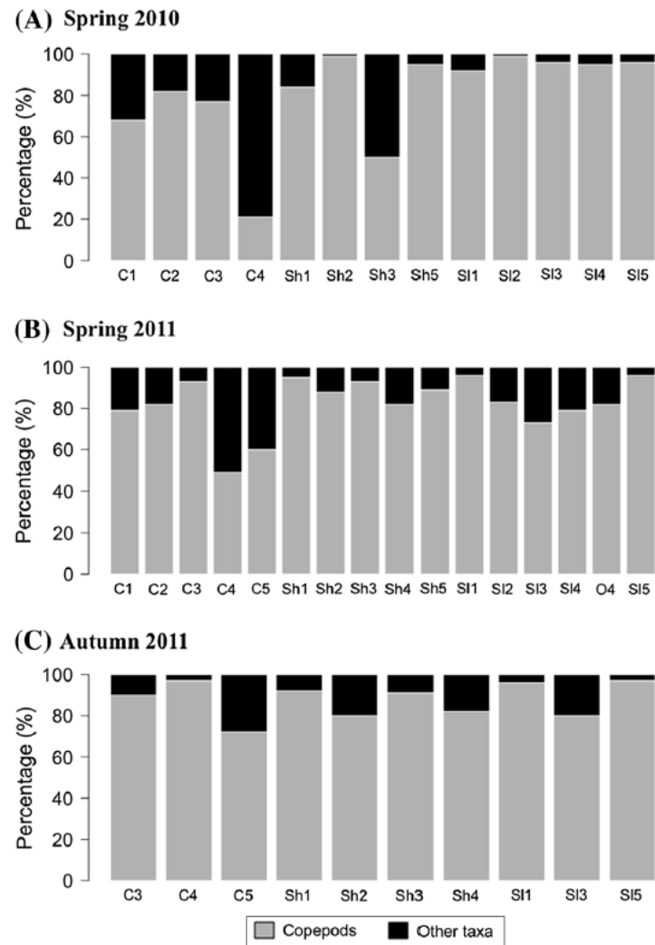
Figure 2. Percentage of copepods relative to the total abundance of mesozooplanktonic organisms (in number of individuals / m 3 ) for each station selected and considered for taxonomic identification in spring 2010, spring 2011 and autumn 2011.
