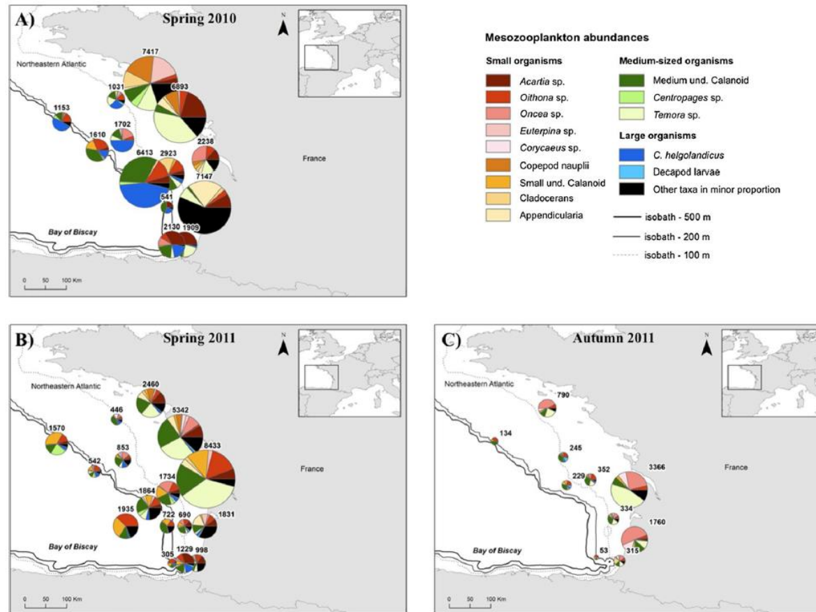
Figure 3. Results of the taxonomic identification performed on mesozooplankton samples collected in a spring 2010, b spring 2011 and c autumn 2011. The number above a pie corresponds to the total abundance of organisms within a station (in number of individuals m^{-3} ), and the size of pies is proportional to the total abundance. Among the ‘dominant taxa’ (see text), small organisms are represented in shades of red to yellow , medium-sized organisms in shades of green and large organisms in shades of blue (see Table 1). Within each station, the proportion of taxa in minor proportion (i.e. with an abundance <5\% when taken individually, and therefore not analysed for stable isotope ratios—see text) is indicated in black . The study area represented ( outlines of the box ) extends from 0^{\circ} to 8^{\circ}W and from 43^{\circ}N to 48^{\circ}N ( Source : Etopo1 NOAA—LIENSs—2013. Design and realisation: Cellule Géomatique LIENSs—UMR 7266)
