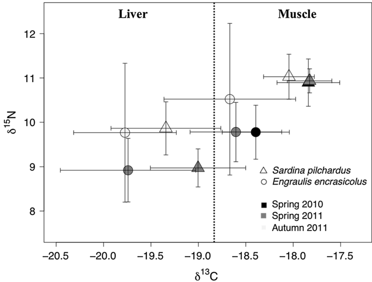
Figure 5. \delta^{13}\text{C} and \delta^{15}\text{N} values (mean \pm SD, in ‰) for European sardine Sardina pilchardus and European anchovy Engraulis encrasicolus , depending on the period considered and on the tissue analysed. Detailed results of statistical tests for significant difference between species or between periods for a given tissue or for a given element are presented in Table 3. The dotted line is only drawn as a guide to visually distinguish muscle and liver tissue values that are presented here on the same figure
