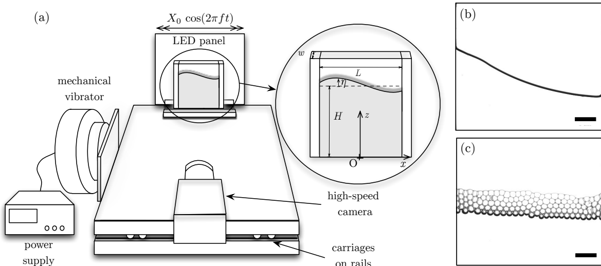
Figure 1: (a) Schematic of the experimental setup. Example of visualization for (b) a Newtonian fluid and for (c) a Newtonian fluid with a 2D liquid foam on the top. The images are recorded at the maximum amplitude of the oscillation. Scale bars are 1 cm.
