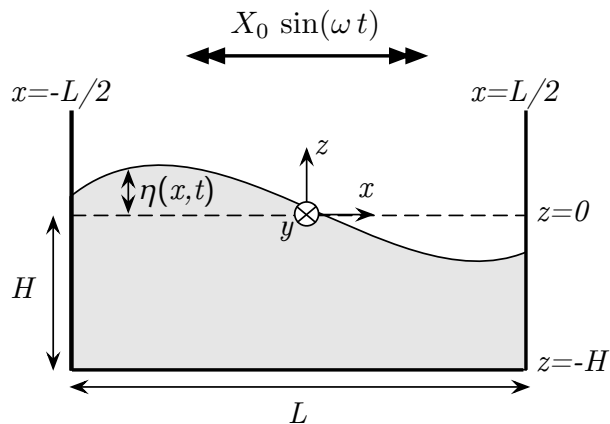
Figure 7: Two-dimensional schematic of the sloshing dynamics in a rectangular container.
