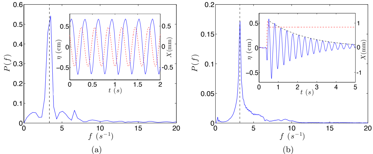
Figure 2: Temporal spectrum P(f) of the free-surface displacement measured 1 cm away from the edge of the cell for (a) a continuous sinusoidal forcing at frequency f=3.3 Hz and (b) an impulse excitation. The vertical dashed line shows the first resonant frequency f_1 \simeq 3.2 Hz. Insets: the corresponding time evolution of the free surface \eta is represented by a blue continuous line (scale: left axis). The red dotted line shows the motion of the container X(t) (scale: right axis). The black dash-dotted line in the inset of (b) corresponds to an exponential damping, \eta_0 \exp(-t/\tau_\ell) , where \eta_0 and 1/\tau_\ell are fitting parameters. Experiments are performed with a depth H = 4 cm of foaming solution in a container of width w = 1.59 cm and length L = 7 cm.
