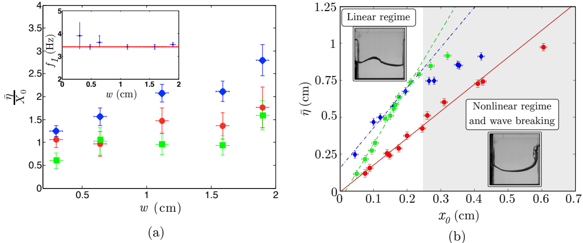
Figure 8: (a) Rescaled maximum amplitude \bar{\eta}/X_0 averaged over x as a function of the width of the cell w for a forcing frequency f = 4 Hz (blue diamonds), f = 5 Hz (red circles) and f = 7 Hz (green squares). Inset: evolution of the first resonant frequency f_1 as a function of w . (b) Maximum amplitude of sloshing \bar{\eta} averaged over x as a function of the amplitude of the moving stage X_0 for a frequency f = 3.1 Hz and a width w = 0.3 cm (green squares), a frequency f = 3.5 Hz and a width w = 1.6 cm (blue diamonds) and a frequency f = 4.8 Hz and a width w = 1.6 cm (red circles).
