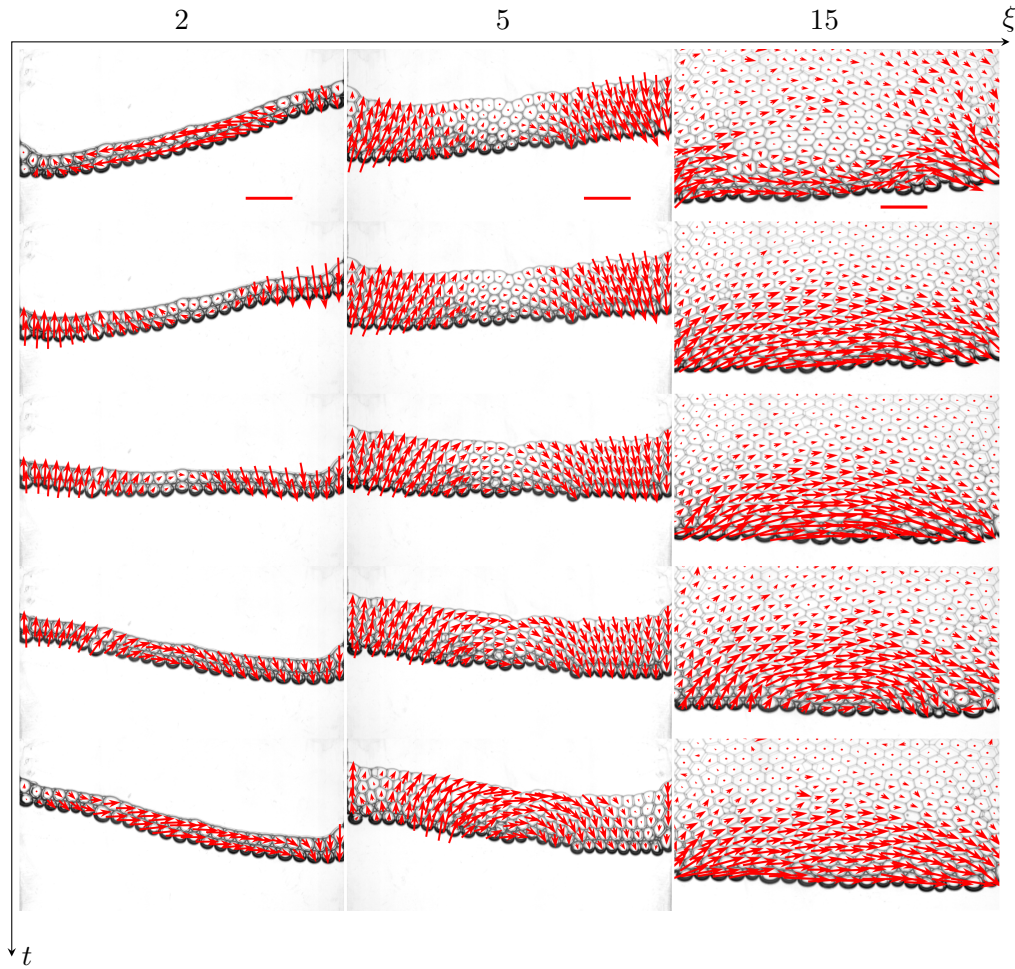
Figure 4: Time evolution of the amplitude of sloshing for a harmonic lateral forcing at f_1 = 3.125 Hz (first resonant frequency) and an amplitude of excitation X_0 = 0.1 cm. The number of layers of bubbles \xi increases from left to right. The arrows indicate the velocity field. The photographs are taken at different moments during half a period of the container oscillation. Scale bars are 1 cm. (Multimedia View).
