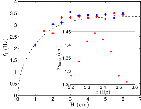
Figure 9: Evolution of the resonant frequency f_1 as a function of the water depth H for a container of length L = 7 cm and two widths: w = 1.59 cm (in blue squares) and w = 0.30 cm (red circles). The dashed line shows the analytical expression of the first resonant frequency f_1 . Inset: evolution of the maximum amplitude of sloshing \eta_{max} for forcing close to the resonant frequency.
