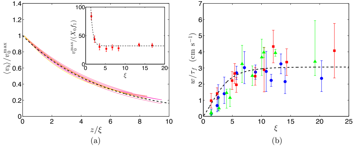
Figure 6: (a) Velocity of the bubbles v_b averaged over one period and normalized by v_0^{max} = v_b(z/\xi = 0) as a function of the vertical position z/\xi in a foam made of 9 layers of bubbles. The curves correspond to different locations x and the black dotted line is the exponential fit \exp[-z/(5.2\xi)] . Inset: Evolution of the rescaled maximum value of the mean velocity of the bubbles v_0^{max}/(X_0 f_1) as a function of \xi . The dotted line corresponds to an exponential fit of the experimental measurements. These measurements are obtained in a w = 0.3 cm wide cell of length L = 7 cm and a height of foaming solution H = 4 cm. (b) Rescaled damping coefficient w/\tau_f as a function of \xi for various widths of the cell: w = 0.3 cm (blue circles), w = 0.6 cm (green triangles) and w = 1.6 cm (red squares) in L = 7 cm cells. The black dashed line shows the best fit adjusting the prefactor in the equation (14).
