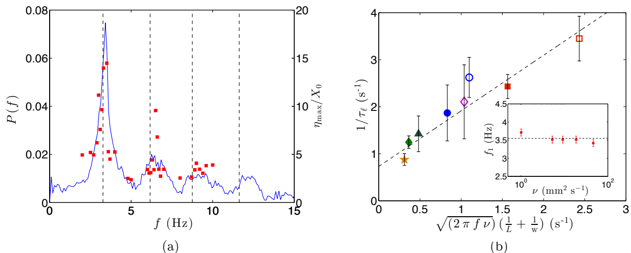
Figure 3: (a) Temporal spectrum P(f) of the surface displacement resulting from an impulse excitation (blue continuous line, left axis), and with a harmonic excitation at a given frequency (red squares, right axis). The vertical dashed lines are the resonant frequencies from equation (1). The experiments are performed with a depth H = 4 cm of water in a container of width w = 1.59 cm and length L = 7 cm. (b) Evolution of the damping coefficient 1/\tau_\ell for w = 1.6 cm and \nu = 5.26 \text{ mm}^2 \text{ s}^{-1} (blue filled circle), w = 1.6 cm and \nu = 9.17 \text{ mm}^2 \text{ s}^{-1} (blue hollow circle), w = 1.6 cm and \nu = 18.6 \text{ mm}^2 \text{ s}^{-1} (red filled square), w = 1.6 cm and \nu = 46.3 \text{ mm}^2 \text{ s}^{-1} (red hollow square), w = 1.6 cm and \nu = 1.01 \text{ mm}^2 \text{ s}^{-1} (green filled diamond), w = 0.48 cm and \nu = 1.01 \text{ mm}^2 \text{ s}^{-1} (purple hollow diamond), w = 1.1 cm and \nu = 1.01 \text{ mm}^2 \text{ s}^{-1} (green filled triangle), w = 1.9 and \nu = 1.01 \text{ mm}^2 \text{ s}^{-1} cm (orange filled star). Inset: first resonance frequency as a function of the kinematic viscosity \nu .
