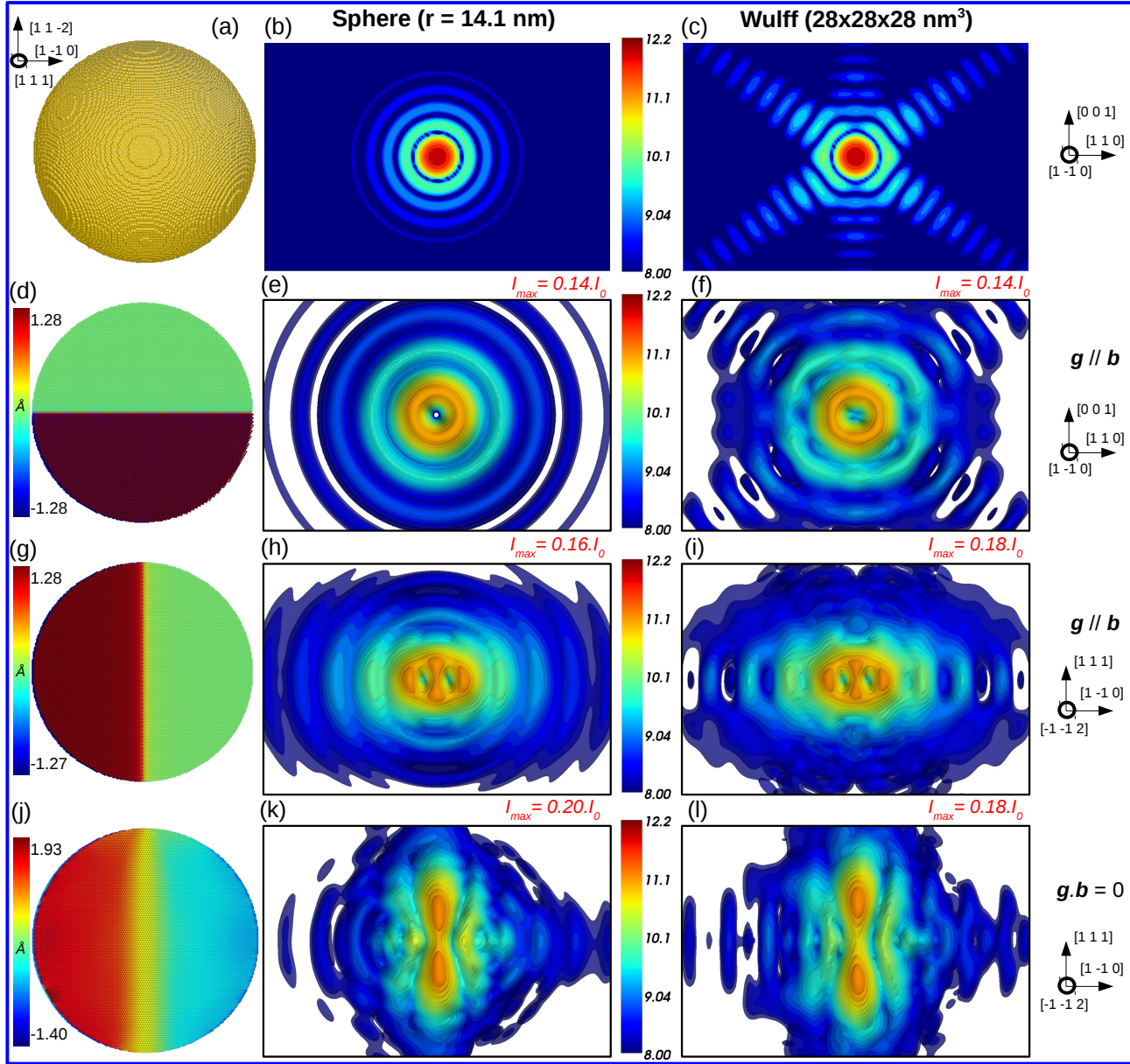
Fig. 9: a) Defect free copper spherical crystal with r = 14.1\text{nm} . Corresponding CXD patterns with \mathbf{g} // \mathbf{b} ( \mathbf{g} = 2\ \bar{2}\ 0 ) for the sphere (b) and the reference copper crystal in Wulff geometry (c). (d) Perfect screw dislocation with \mathbf{b} = \frac{1}{2} [1\ \bar{1}\ 0] at the centre of the section in the same spherical crystal. The colour scale shows the u_x component of the atomic displacement field. Corresponding CXD patterns with \mathbf{g} // \mathbf{b} ( \mathbf{g} = 2\ \bar{2}\ 0 ) for a sphere (e) and a Wulff crystal (f). (g) Perfect edge dislocation with \mathbf{b} = \frac{1}{2} [1\ \bar{1}\ 0] in the same crystal. Corresponding CXD patterns with \mathbf{g} // \mathbf{b} ( \mathbf{g} = 2\ \bar{2}\ 0 ) for a sphere (h) and a Wulff crystal (i). (j) Dissociation of the perfect dislocation in 2 Shockley partials in the (1\ 1\ 1) plane with \mathbf{b}_{p1} = 1/6[1\ \bar{2}\ 1] and \mathbf{b}_{p2} = 1/6[2\ \bar{1}\ 1] in the same crystal. Corresponding CXD patterns with \mathbf{g} \cdot \mathbf{b} = 0 ( \mathbf{g} = 2\ 2\ 4 ) for a sphere (k) and a Wulff crystal (l). The selected area of the reciprocal space is kept to the same value in all figures and is equal to 0.45 \times 0.675\ (1/\text{\AA})^2
