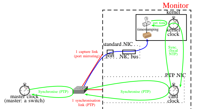
Figure 6. Experimental timestamping mechanism
