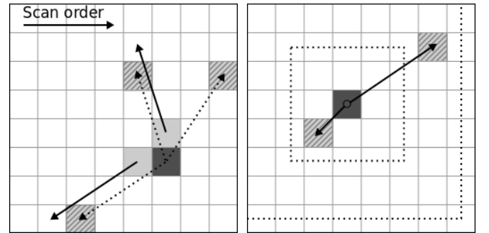
(a) Propagation. Plain arrows are the current patch offsets. The dotted current patch offsets. The dotted ar-squares represent the successive rows are the offsets that are checked windows used to search a good approximate neighbor.
