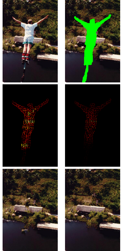
Fig. 7. Illustration of the proposed data term for the Bungee jumping . Top: the original image and the part we want to remove. Middle: data terms of Criminisi et al. [2] (left) and ours (right) with a heat color map (dark red for low data term values, and yellow for high values). Bottom: resulting inpainted images. Due to the dilation effect of the original data term (Eq. 4), the roof of the shelter is broken (left). One can see also some texture garbage on the water. The proposed data term (Eq. 12) concentrates on the interface between the roof of the shelter and the jumper and avoids the copy of a forest-only patch onto the roof. Similar results with state-of-the-art data terms can be found in Fig.4.
