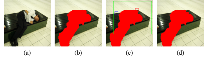
Fig. 2. Illustration of one iteration of the greedy approach [2]. (a) Original Image. (b) Masked image. (c) Search for the best patch. The target patch is depicted in red, the lookup area in green, and the best patch in blue. (d) Result after pasting the blue patch of (c).
