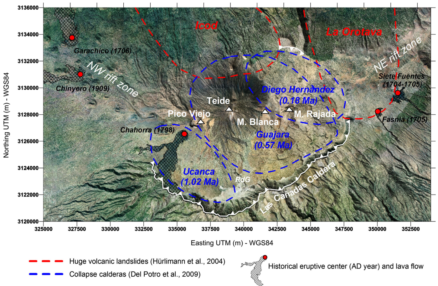
Fig. 2. Orthophoto of the studied area in central Tenerife superimposed over IGN Digital Elevation Model (cell size 25 m), showing also historical eruptive centers and lava flows, main central volcanic edifices, Las Cañadas caldera wall and the proposed boundaries of collapse calderas (Del Potro et al., 2009) and huge volcanic landslides (Hürlimann et al., 2004). RdG is the Roques de García spur.
