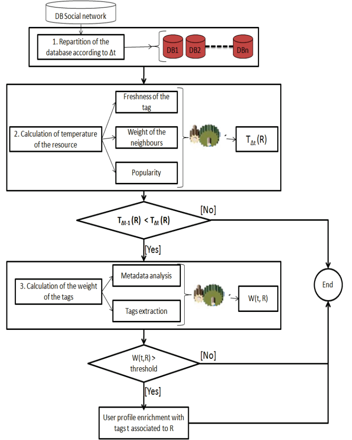
Fig. 4. The process of enriching the social user profile for a \Delta t .
