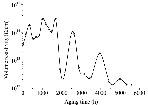
Fig. 5. Volume resistivity evolution versus aging time.
