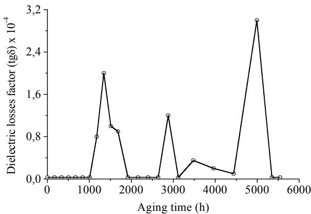
Fig. 1. Dielectric losses factor variations with respect to aging time.
