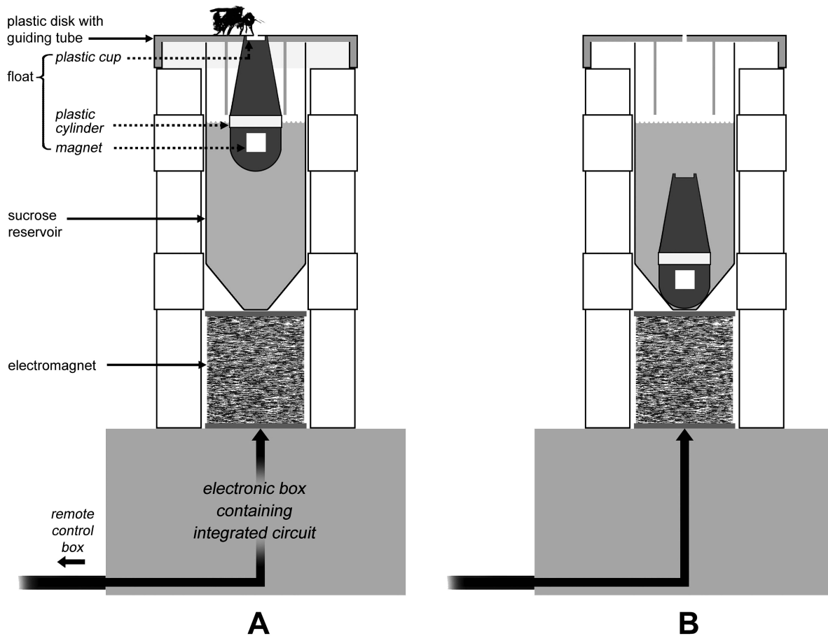
Figure 1: Schematic diagrams of a side view of the artificial flower. The cup containing sucrose solution was refilled at a distance by the experimenter by switching on/off the electromagnet using a remote control box. A , When the electromagnet is switched off, the cup (containing sucrose solution) floats below the hole in the blue plastic disk through which the bee can feed. B , When the electromagnet is switched on, the float is drawn down under the surface of the sucrose solution, which acts to fill the cup. Illustration by S. Blackburn.
