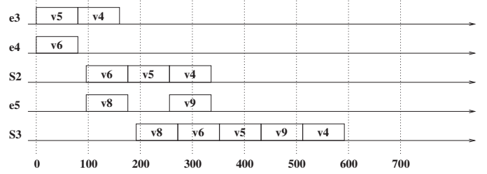
Fig. 5. Worst-case scenario for v_4 with priority 3
