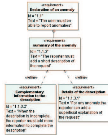
Fig. 3. Snapshot of the BTS requirements model
