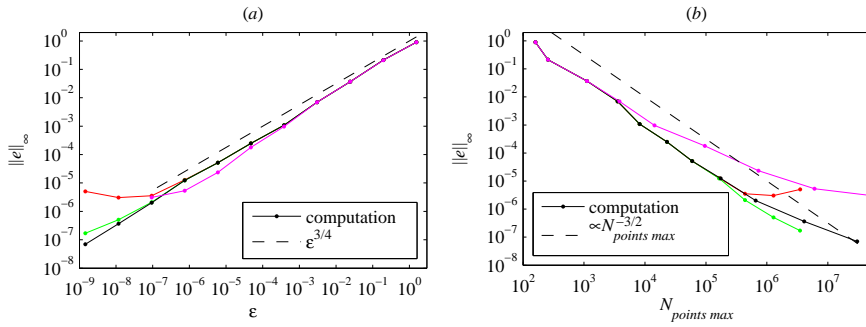
Fig. 15 Convergence tests. Decay of the L^\infty error (a) versus \varepsilon and (b) versus the maximum number of grid points N_{points\ max} . Different colours correspond to different values of \eta : \eta = 10^{-5} (red), 10^{-6} (green), 10^{-7} (black), 10^{-8} (magenta).
