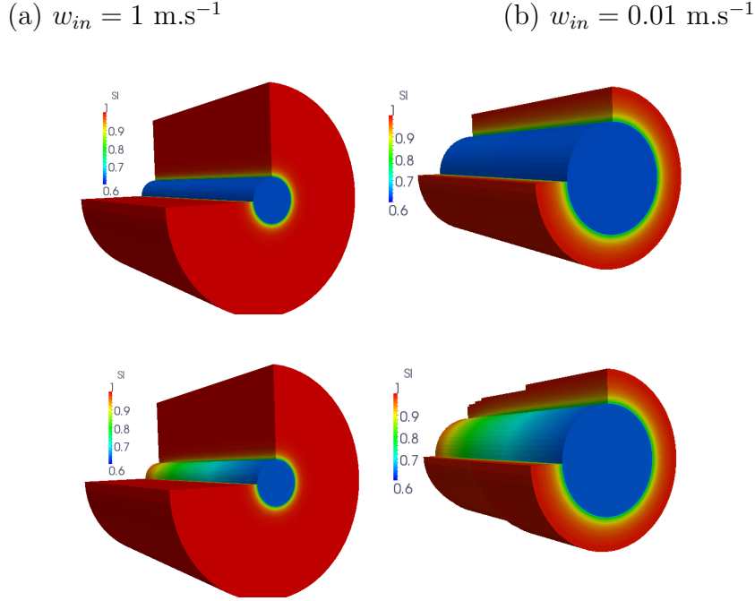
Figure 7: Stationary liquid saturation s^l obtained for w_{in} = 1 \text{ m.s}^{-1} (a) and for w_{in} = 0.01 \text{ m.s}^{-1} (b). The bottom figures zoom the liquid saturation in the porous medium below the threshold value 0.99. In the gallery the liquid saturation corresponds to the saturation at the interface function of x .
