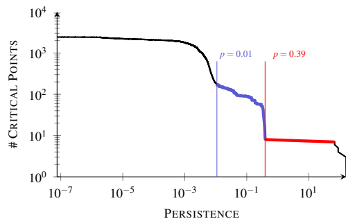
(b) Persistence curve highlighted with two different simplification levels (blue and red line).
