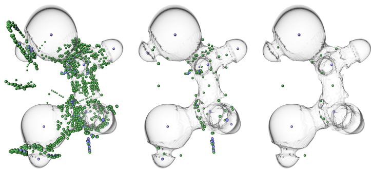
(a) Minima (blue) and 1-saddles (green) for three simplification levels: no simplification (left), p = 0.01 (middle), p = 0.39 (right).
