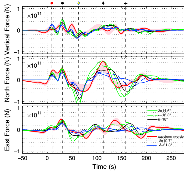
Figure 14. Sensitivity of the force-time function to the rockslide friction coefficient. The lines correspond to \delta = 14.6^\circ , (green) 16.3^\circ (dashed green), 18^\circ (black), 19.7^\circ (dashed blue), and 21.3^\circ (blue). The red line corresponds to the best inverted force and the pink area is the confidence interval. The markers represents the peaks of the force analyzed in Figure 15.
