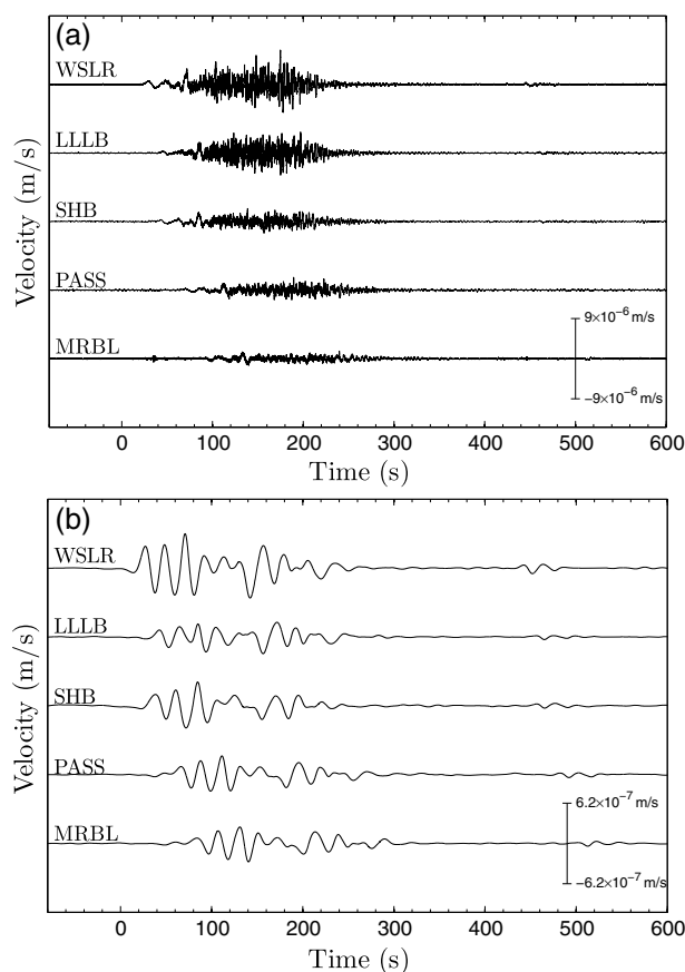
Figure 2. (a) Raw and (b) 20–150 s filtered vertical component of the seismic signal recorded at five stations used to perform the waveform inversion. The location of the stations are shown in Figure 1a.
