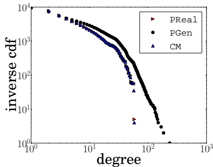
Figure 5: Inverse cumulative degree distribution
