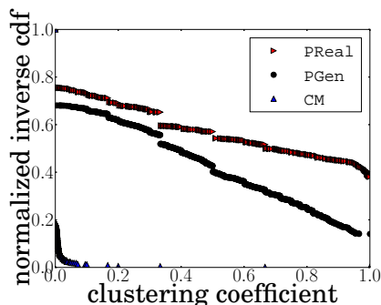
Figure 6: Clustering coefficient inverse cumulative distribution
