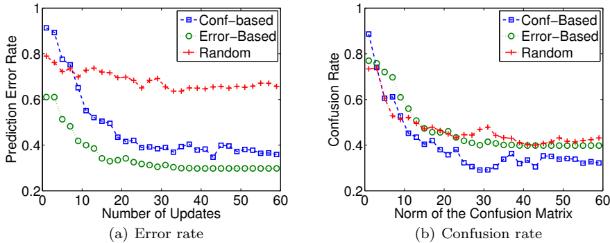
Fig. 5: Error and confusion risk on Reuters dataset with various update strategies.
