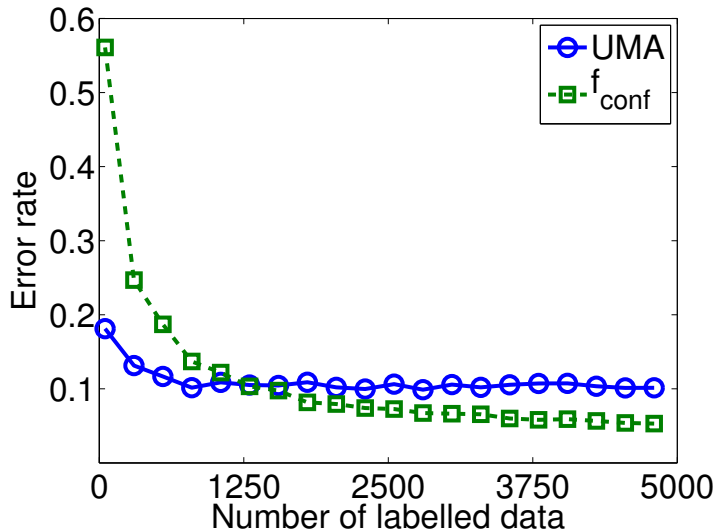
Fig. 3: Error rate of UMA and f_{\text{conf}} with respect to the sampling size. Reuters dataset with m = 70 for the sake of figure’s readability.
