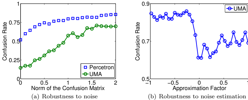
Fig. 1: (a) evolution of the confusion rate (y-axis) for different noise levels (x-axis); (b) evolution of the same quantity with respect to errors in the confusion matrix C (x-axis) measured by the approximation factor (see text).
