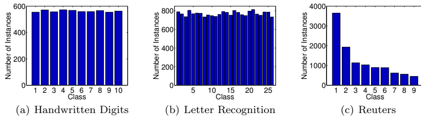
Fig. 2: Class distribution for the three datasets.
