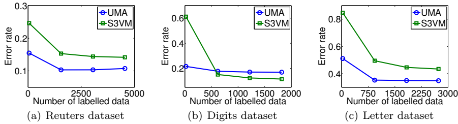
Fig. 4: Error rates for the Reuter (left), optical digit recognition (center) and letter (right) datasets with respect to the size of \mathcal{S}_{\text{conf}} . Average over 15 runs.
