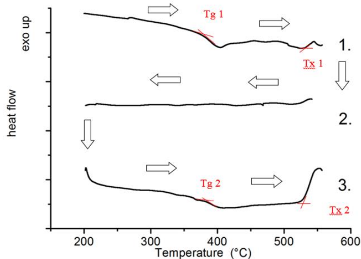
Figure 1: DSC analysis of 20\text{Ga}_2\text{S}_3\text{-65GeS}_2\text{-15CsCl}
