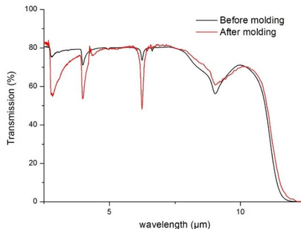
Figure 6: Transmission of the 20\text{Ga}_2\text{S}_3\text{-}65\text{GeS}_2\text{-}15\text{CsCl} before and after molding
