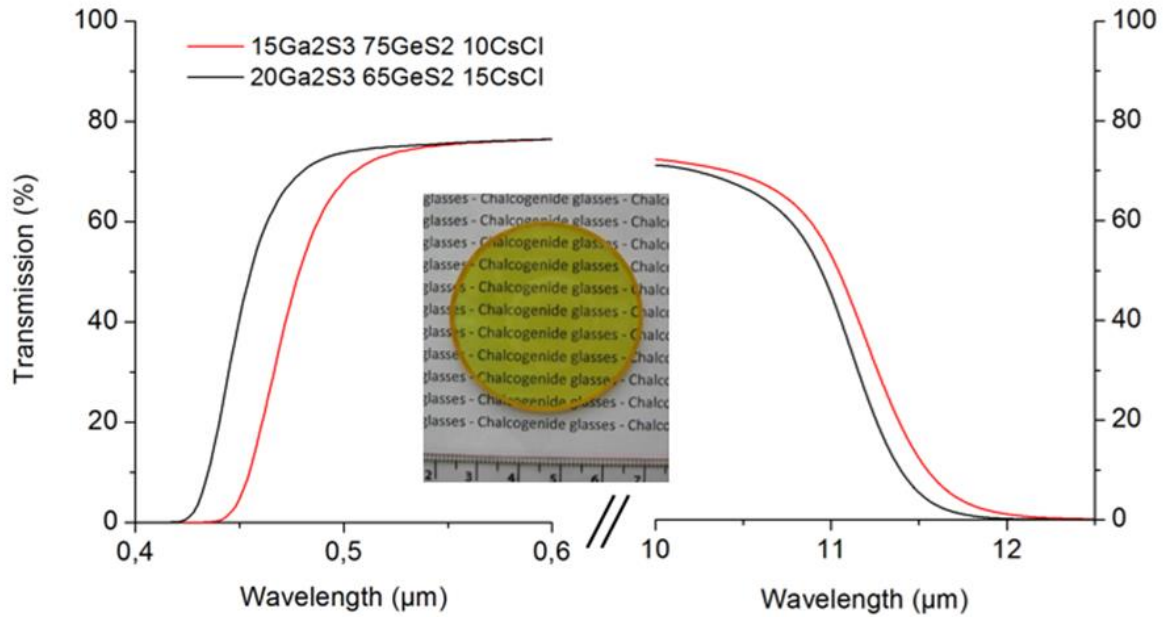
Figure 2: Comparison of 15 Ga 2 S 3 75 GeS 2 10 CsCl and 20 Ga 2 S 3 65 GeS 2 15 CsCl transmissions and a picture of the second composition with a 45mm diameter
