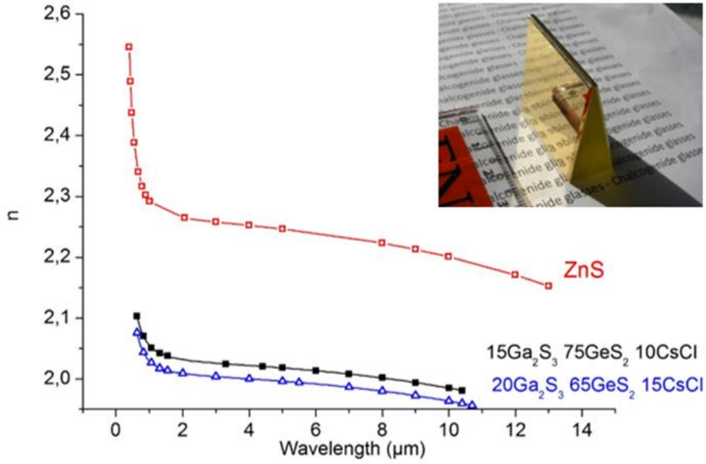
Figure 3: Refractive index of the two glasses compositions and ZnS, the photograph shows the 20Ga 2 S 3 -65GeS 2 -15CsCl prism used for refractive index measurements
