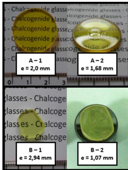
Figure 5: Molding of the compositions 15\text{Ga}_2\text{S}_3\text{-}75\text{GeS}_2\text{-}10\text{CsCl} (aspherical shape: A-1 and A-2) and 20\text{Ga}_2\text{S}_3\text{-}65\text{GeS}_2\text{-}15\text{CsCl} (flat shape: B-1 and B-2)
