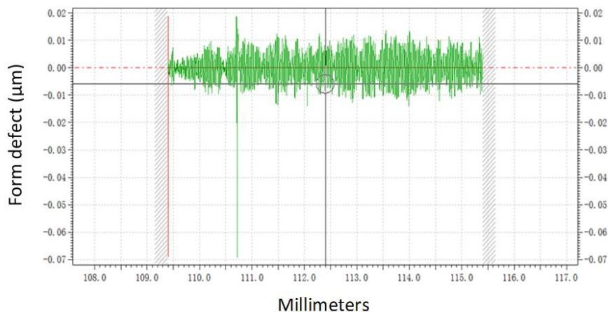
Figure 7: Control of the roughness of the aspherical shape
