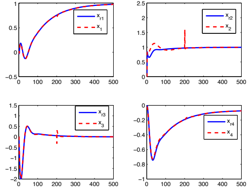
Fig. 2. The fault-tolerant result in a partial loss of effectiveness fault scenario
