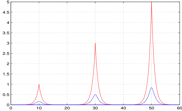
Figure 1: Sum of three red peakons \sum_{i=1}^3 (2i-1)\varphi[x - 10(2i-1)] and three blue smooth-peaks \sum_{i=1}^3 (2i-1)\rho[x - 10(2i-1)] (at time t = 10 with respective speeds 1, 3, 5, and \alpha = 0 ) profiles.
