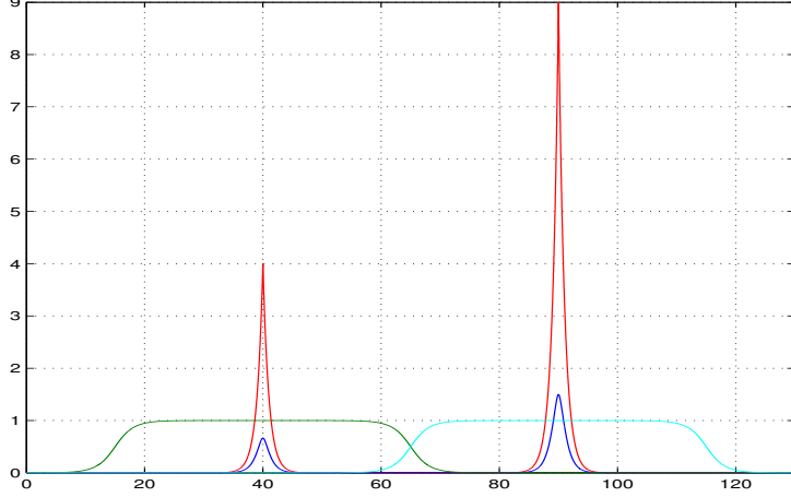
Figure 4: Localization-functions \phi_{green}(x) = \psi(x - 15) - \psi(x - 65) , \phi_{cyan}(x) = \psi(x - 65) - \psi(x - 115) (at time t = 10 ) profiles. Also the sum of two peakons 4\varphi(x - 40) + 9\varphi(x - 90) and two smooth-peakons 4\rho(x - 40) + 9\rho(x - 90) (at time t = 10 , with respective speeds 4, 9, and \alpha = 0 ) profiles. In this example, one can see that \phi_{green} (respectively \phi_{cyan} ) is close to 1 in ]25, 55[ (respectively in ]75, 105[ ) and decays exponentially in \mathbb{R} \setminus ]10, 70[ (respectively in \mathbb{R} \setminus ]60, 120[ ).
