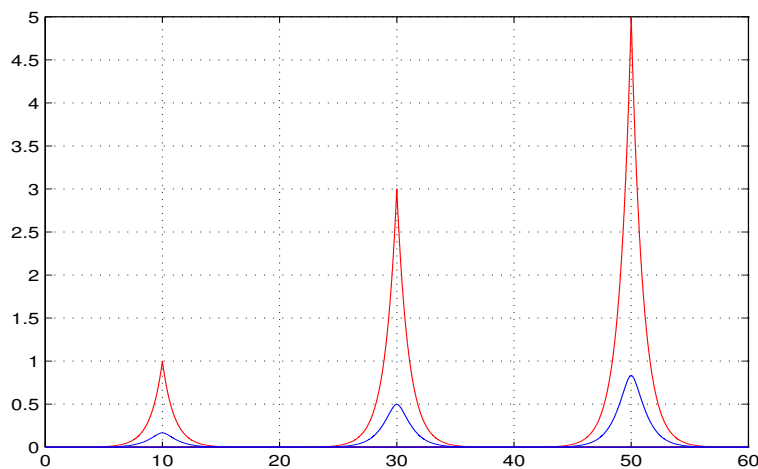
Figure 1: Sum of three red peakons \sum_{i=1}^3 (2i-1)\varphi[x-10(2i-1)] and three blue smooth-peaks \sum_{i=1}^3 (2i-1)\rho[x-10(2i-1)] (at time t=10 with respective speeds 1, 3, 5, and \alpha=0 ) profiles.
