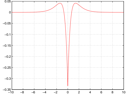
(c) \rho''(x) profile
