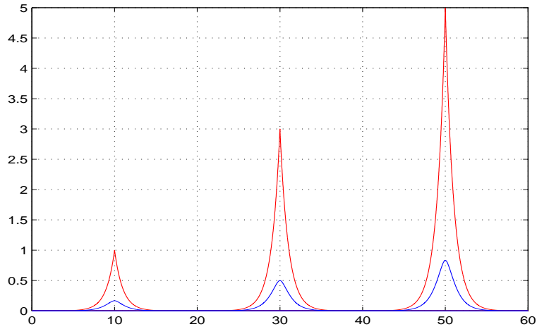
Figure 1: Sum of three red peaks \sum_{i=1}^3 (2i-1)\varphi[x-10(2i-1)] and three blue smooth-peaks \sum_{i=1}^3 (2i-1)\rho[x-10(2i-1)] (at time t=10 with respective speeds 1, 3, 5, and \alpha=0 ) profiles.
