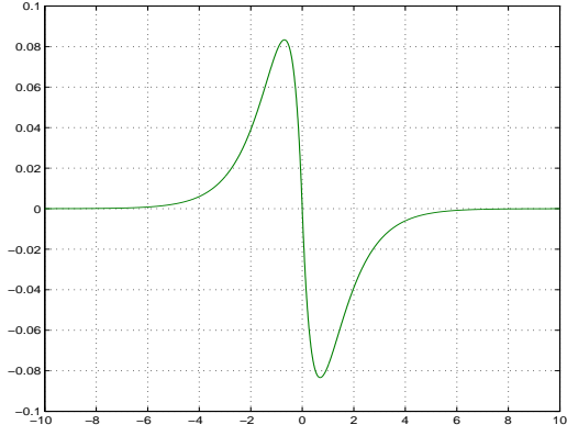
(b) \rho'(x) profile.
