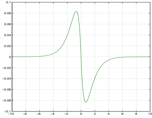
(b) \rho'(x) profile.
