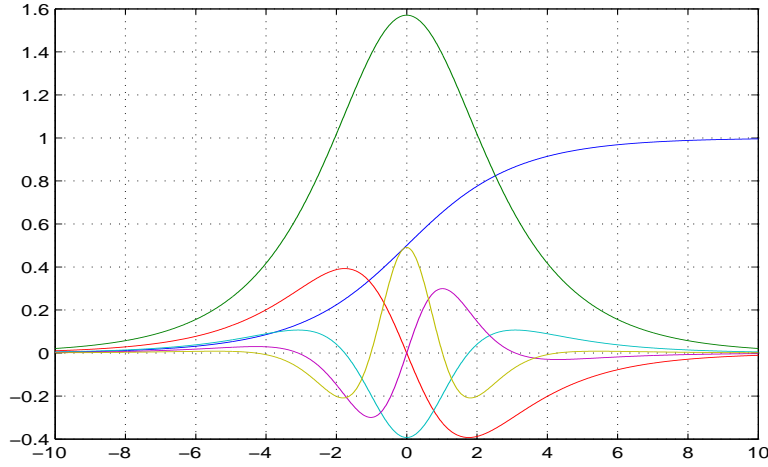
Figure 3: \psi^{(q)}(x) , q = 0, 1, 2, 3, 4, 5 , profiles.
