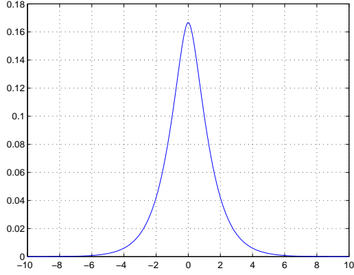
(a) \rho(x) profile.
