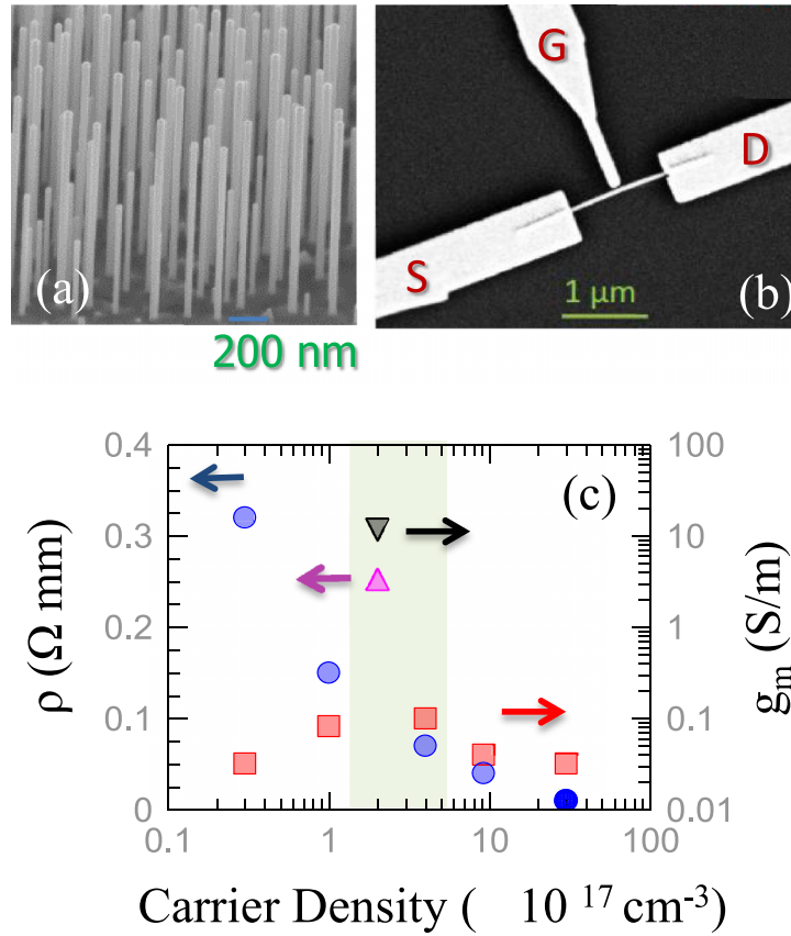
FIG. 1. (a) 45° tilted scanning electron micrograph (SEM) image of a forest of InAs nanowires having a length of about 1.5 \mu\text{m} , an average diameter 2r=35 \text{ nm} , and grown with DtBSe precursor line pressures of 0.1 Torr. (b) SEM image of a FET based on an InAs NW. (c) Peak transconductance (red squares) normalized to the gate length ( g_m ) and resistivity ( \rho ). Values are plotted as a function of extracted carrier density in the transistor channel; the black and pink triangles correspond to the g_m and \rho values of device A.
