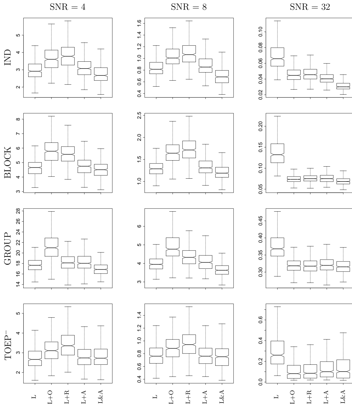
Figure 1: Mean prediction error computed over 500 simulations for each design. Lasso direct estimation (L) is compared to: Lasso screening followed by OLS estimation (L+O), Lasso screening followed by ridge estimation (L+R), Lasso screening followed by adaptive-ridge estimation (L+A), jointly optimized Lasso screening with adaptive-ridge estimation (L&A).
